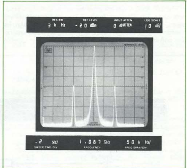
Figure 26. 2% AM
