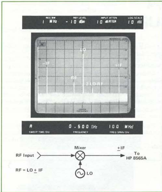
Figure 24. Mixer measurement
