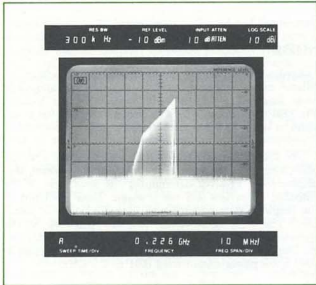
Figure 38. Spurious radiation
